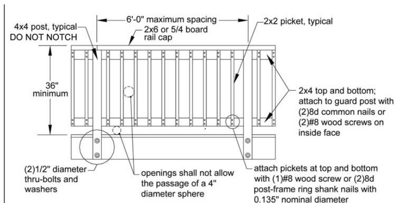
Figure 24: Typical Guard Detail
