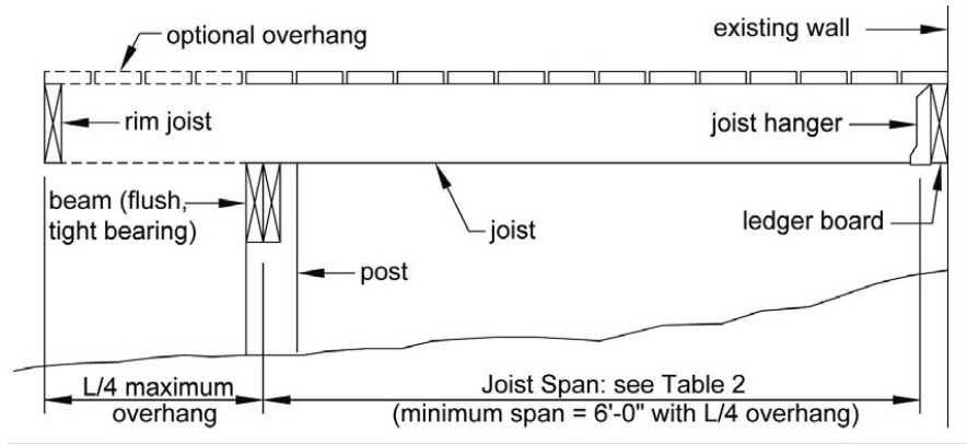
Figure 1A: Joist Span – Deck Attached at House
