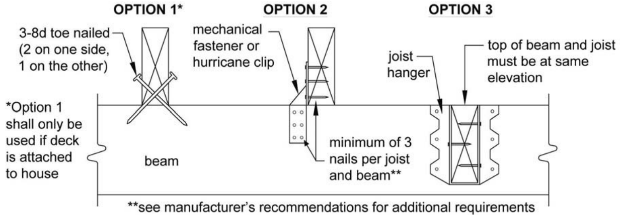
Figure 6: Joist-to-Beam Detail
